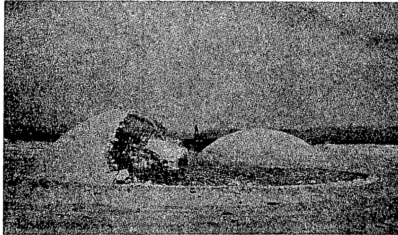
Fig. 13—Left side of responding concrete dome at 70-psi overpressure region.
